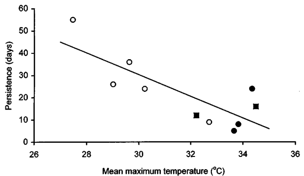
Fig. 3. Effect of temperature on the period for which the knockdown of tsetse remained at or above 50%. Plots distinguish periods with different amounts of average daily rain (○, none; ●, 0.1–0.9 mm; ■, 2.4–3.6 mm), but the regression line (slope significant at P < 0.01 ) is fitted to the pooled data. Details of the regression are given in the text.
